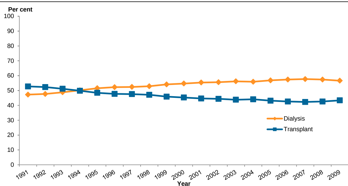
Figure 3.4: Proportion of treated-ESKD patients receiving dialysis or with a functioning kidney transplant, 1991 to 2009
