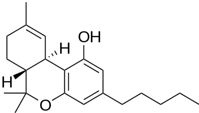
Δ9-Tetrahydrocannabinol (THC)
