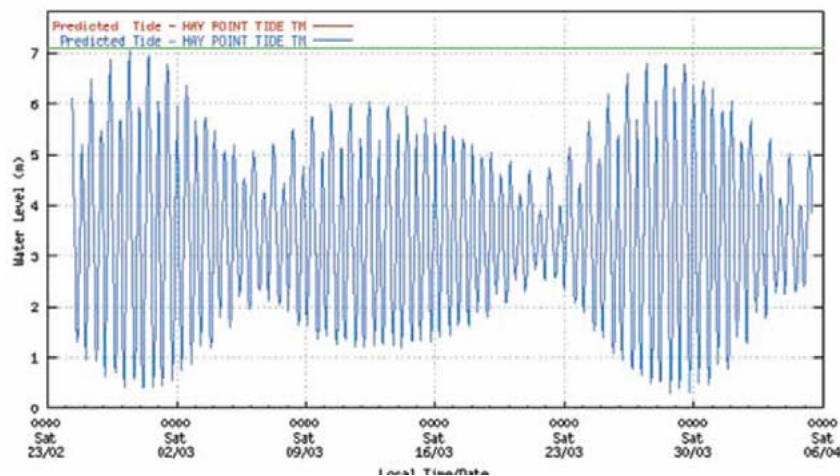
Figure 10 Tidal variations at Hay Point, Queensland. Source: Australian Institute for Disaster Resilience.
