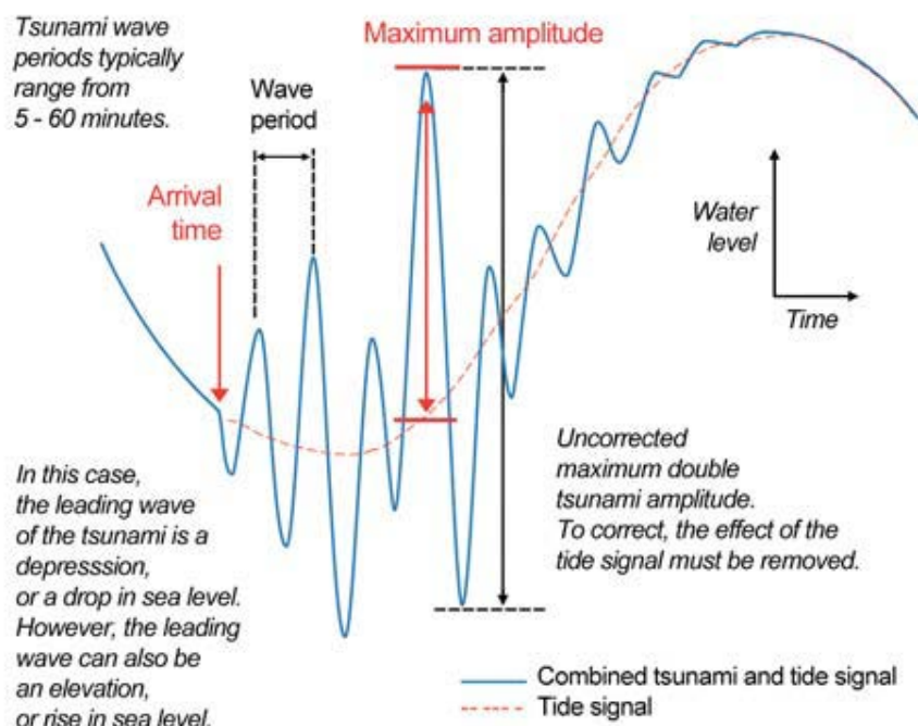
Figure 4 Tsunami wave level over time. Source: Tsunami Glossary, courtesy of International Tsunami Information Center.
