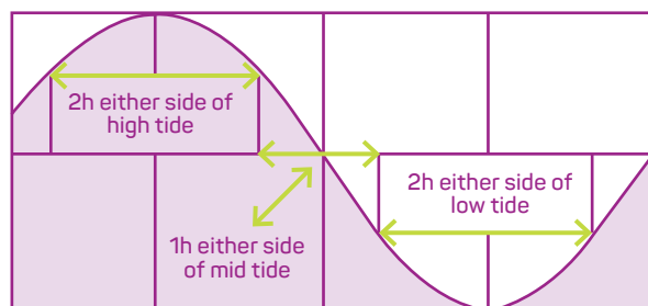
Figure 9 Daily tide cycle. Source: Australian Institute for Disaster Resilience.
