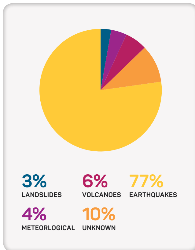
Figure 6 Tsunami event sources based on a historical tsunami event database. Source: Adapted from National Centers for Environmental Information (NCEI, formerly NGDC) of National Oceanic and Atmospheric Administration (NOAA). Image courtesy of Surf Life Saving Australia.
