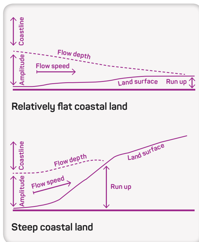
Figure 3 Run-up height and inundation distance on flat coastal land compared to steep coastal land for a tsunami of the same wave amplitude at the coast. Source: Ministry of Civil Defence and Emergency Management, New Zealand, Tsunami Evacuation Zones: Director's Guideline for Civil Defence Emergency Management, at www.civildefence.govt.nz/assets/Uploads/publications/dgl-08-16-Tsunami-Evacuation-Zones.pdf (PDF 4.03MB).
