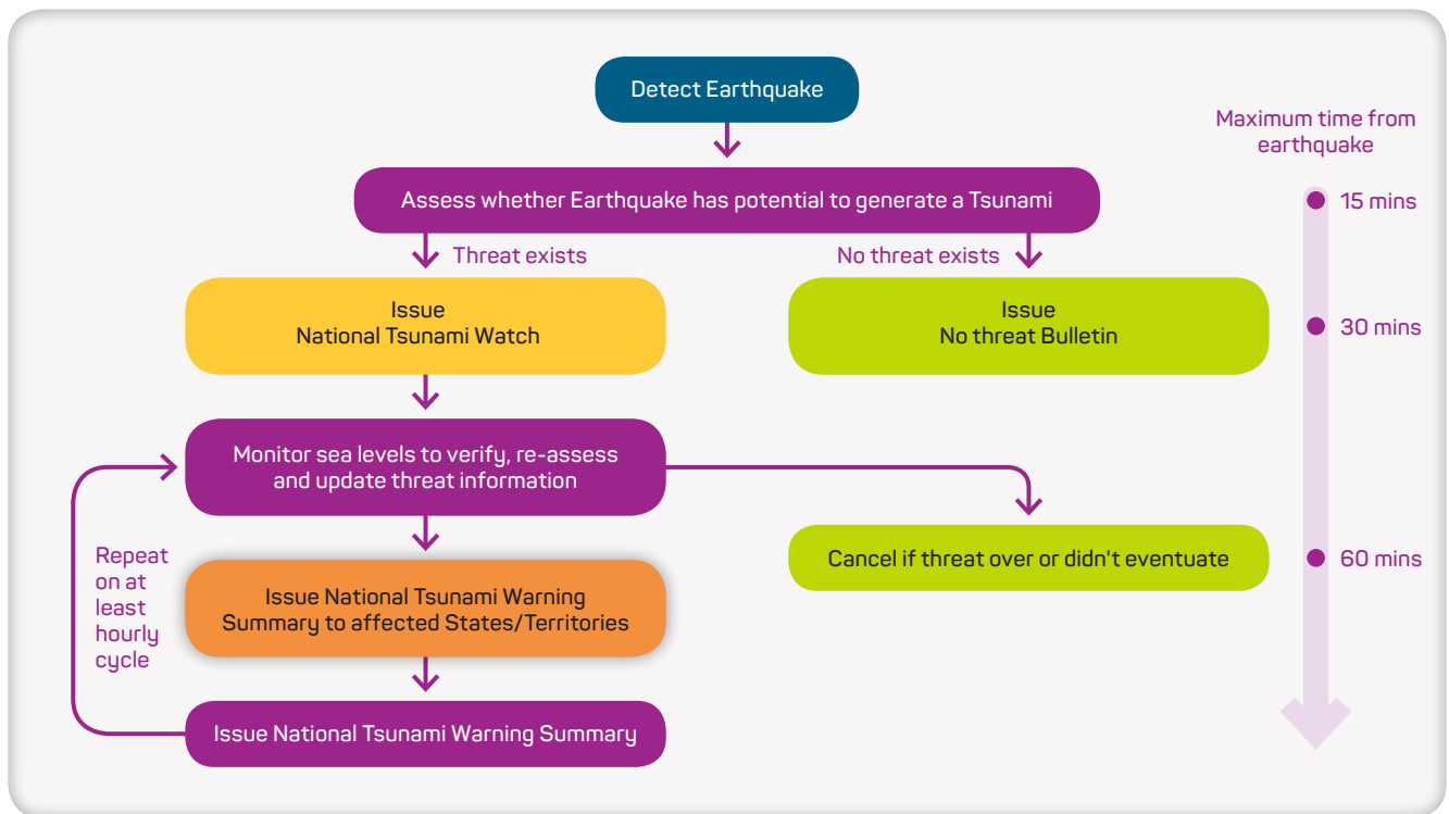
Figure 8 Tsunami warnings and schedule. Source: JATWC. Image courtesy of Bureau of Meteorology, available at www.bom.gov.au/tsunami/about/tsunami_warnings.shtml .
