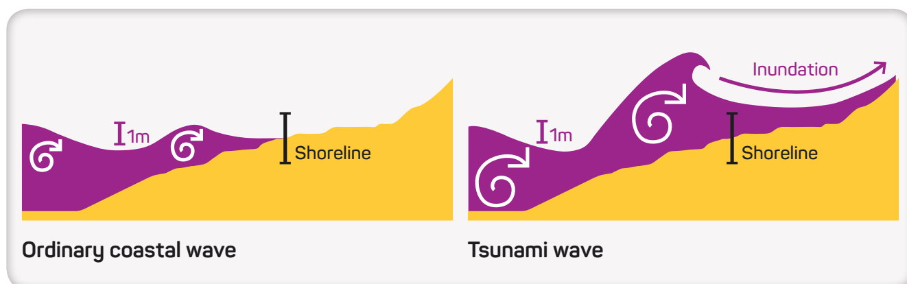
Figure 1 Wave behaviour of a coastal (wind-driven) wave compared to that of a tsunami wave. Source: Ministry of Civil Defence and Emergency Management, New Zealand, Tsunami Evacuation Zones: Director's Guideline for Civil Defence Emergency Management, at www.civildefence.govt.nz/assets/Uploads/publications/dgl-08-16-Tsunami-Evacuation-Zones.pdf (PDF 4.03MB).
