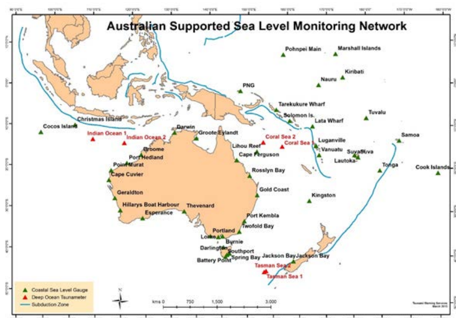
Figure 13 Australian Supported Sea Level Monitoring Network operated by the Bureau; examples of a tide gauges and a DART™ buoy. Source: Images courtesy of Bureau of Meteorology.
