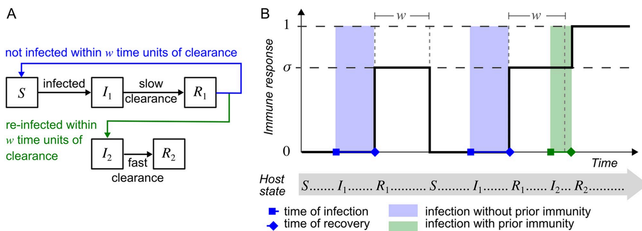
Fig 1. Model of the natural history of disease with respect to a single strain. A: Hosts without prior immunity to a particular strain (S) become infected by contacting infected hosts (I 1 or I 2 ). These infections (I 1 ) clear at an average rate \gamma which confers temporary immunity (R 1 ). This temporary immunity reduces the duration of a subsequent infection (I 2 ) by a factor dependent on the strength of temporary strain-specific immunity ( \sigma ) if the subsequent infection occurs within a short-enough time window (the maximum inter-infection interval, w ) from the time of clearance (green line). If infection does not occur within this time frame (blue line), then temporary immunity wanes and a subsequent infection has the characteristics of a first infection. If temporary immunity does not wane before the next infection, then the clearance of this next infection occurs faster, and confers enduring immunity protecting against further infection (R 2 ). B: An example of a host's immune response (solid black line) following three episodes of infection by the same strain. Here, the temporary immunity acquired following the first infection wanes before the second infection. The clearance of the second infection leads again to temporary immunity. However this becomes enduring immunity following the clearance of the third, more timely, infection.
