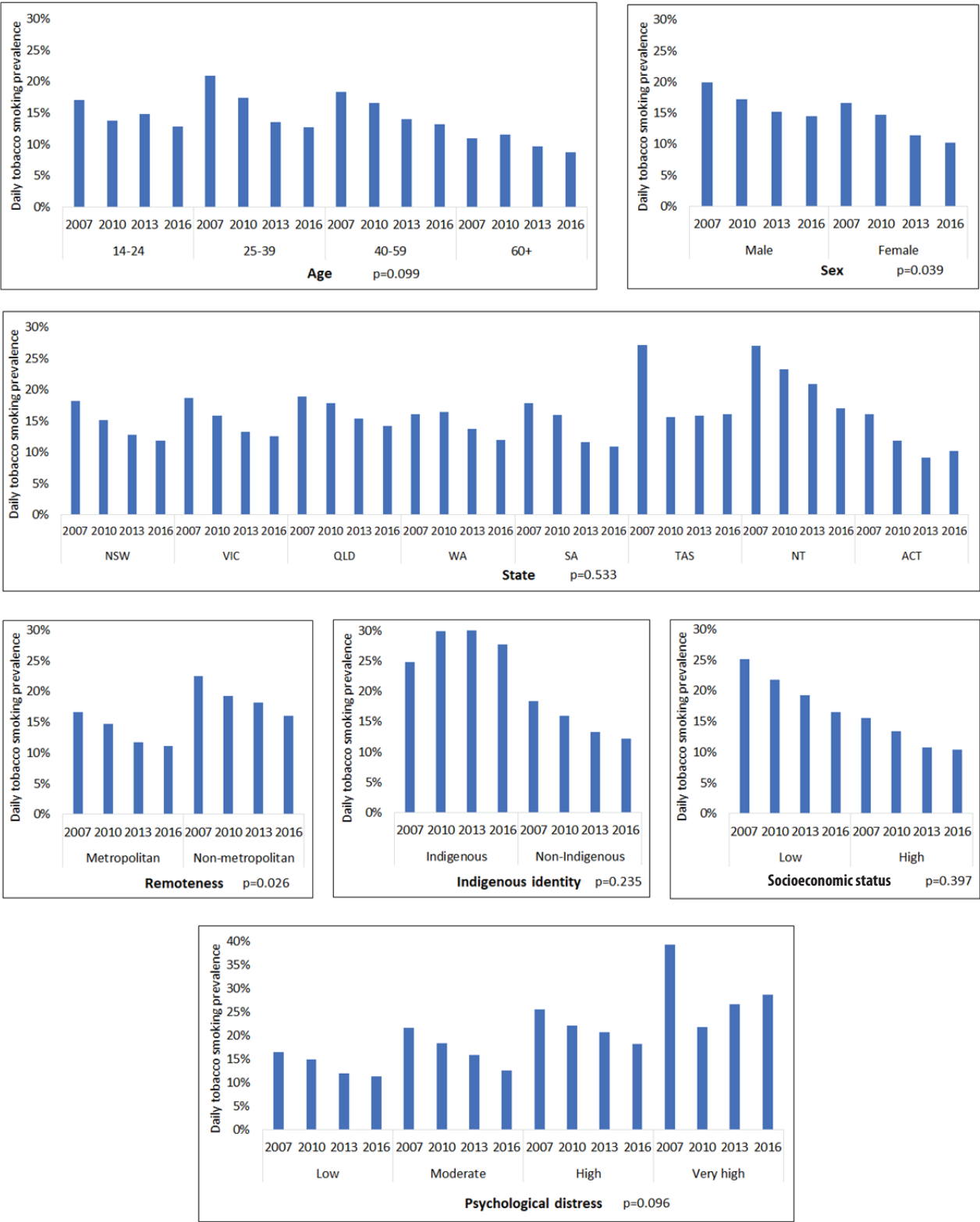
Figure 1: First logistic regression model: Daily smoking prevalence of employed Australians by year and age, sex, state/territory, remoteness, Indigenous identity, socioeconomic status and psychological distress, 2007-2016.
