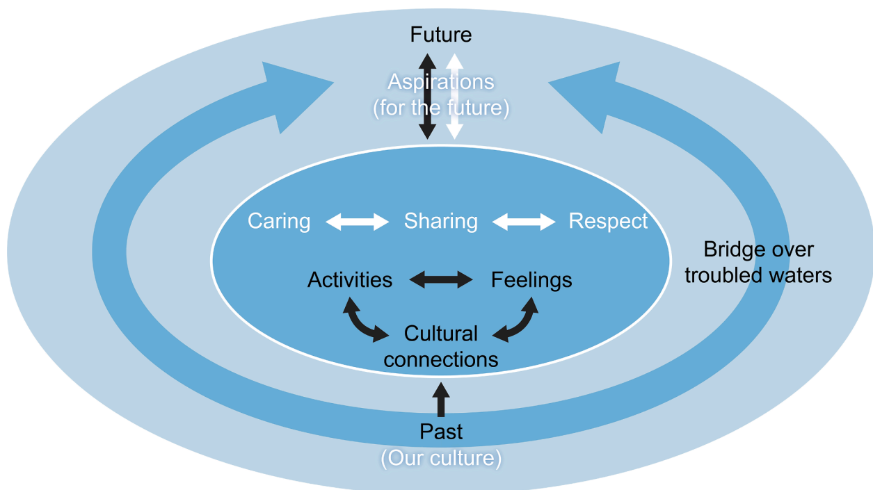
Fig. 2. Mental map of the key themes discussed when talking about (a) ‘connections to Country’ – black text; and (b) ‘what people do for Country’ – white text; arrows represent directions of connections between the themes. Six themes in the oval are all closely connected, and placed in a temporal dimension from past, over present, to future.
