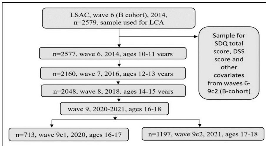
FIGURE 1 Data framework.
